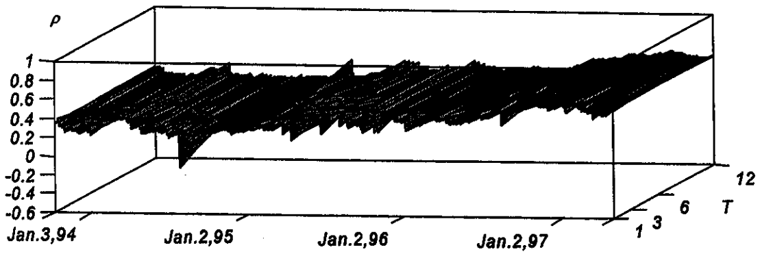
C. \rho(USD_{CHF}, DEM_{CHF})
