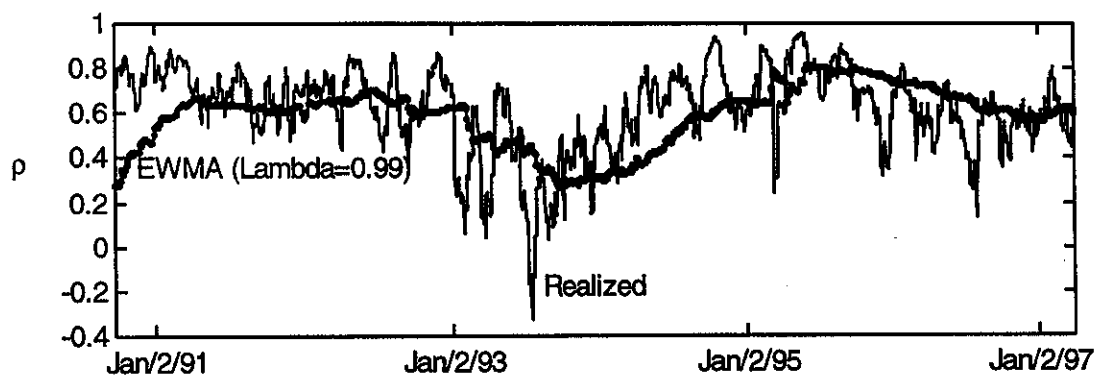
F. Realized and EWMA ( \lambda=0.99 ) Correlation
