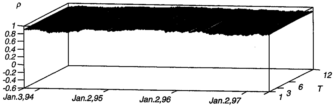
B. \rho(USD_{DEM}, CHF_{DEM})
